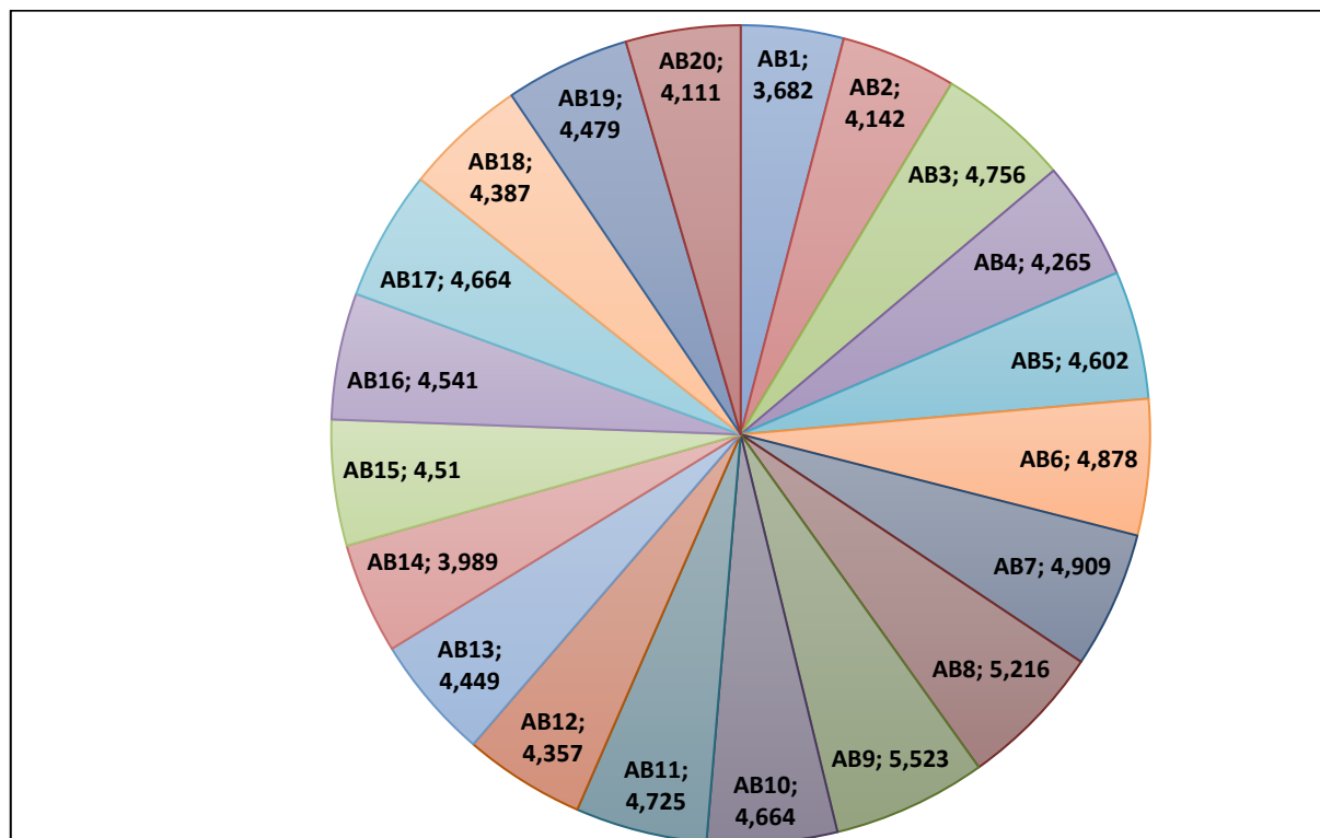
Figure 5. Results of ELCR in all soil samples in the present study.
