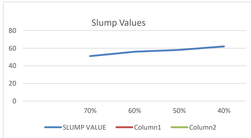
Figure 2: Slump Values
