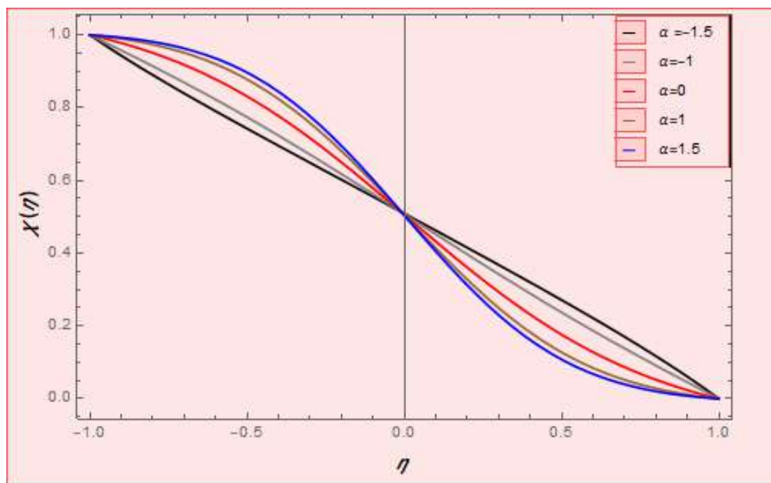
Fig 3; The effect of expansion/contraction ratio parameter on concentration profiles.
