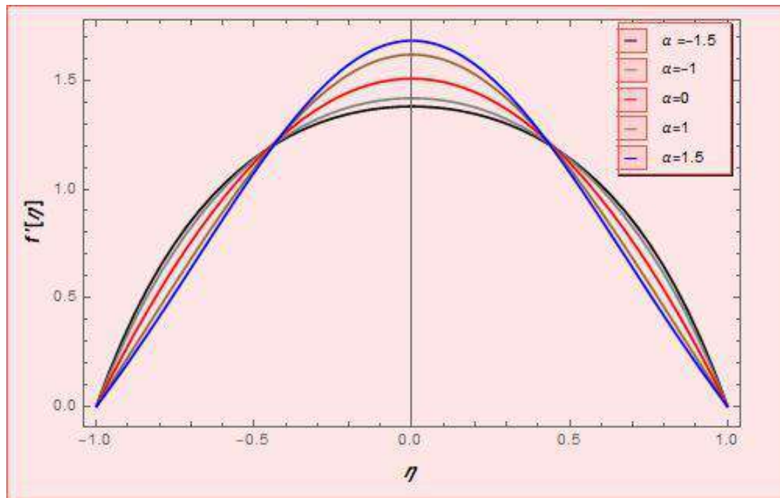
Fig 2; The effect of expansion/contraction ratio parameter on radial velocity
