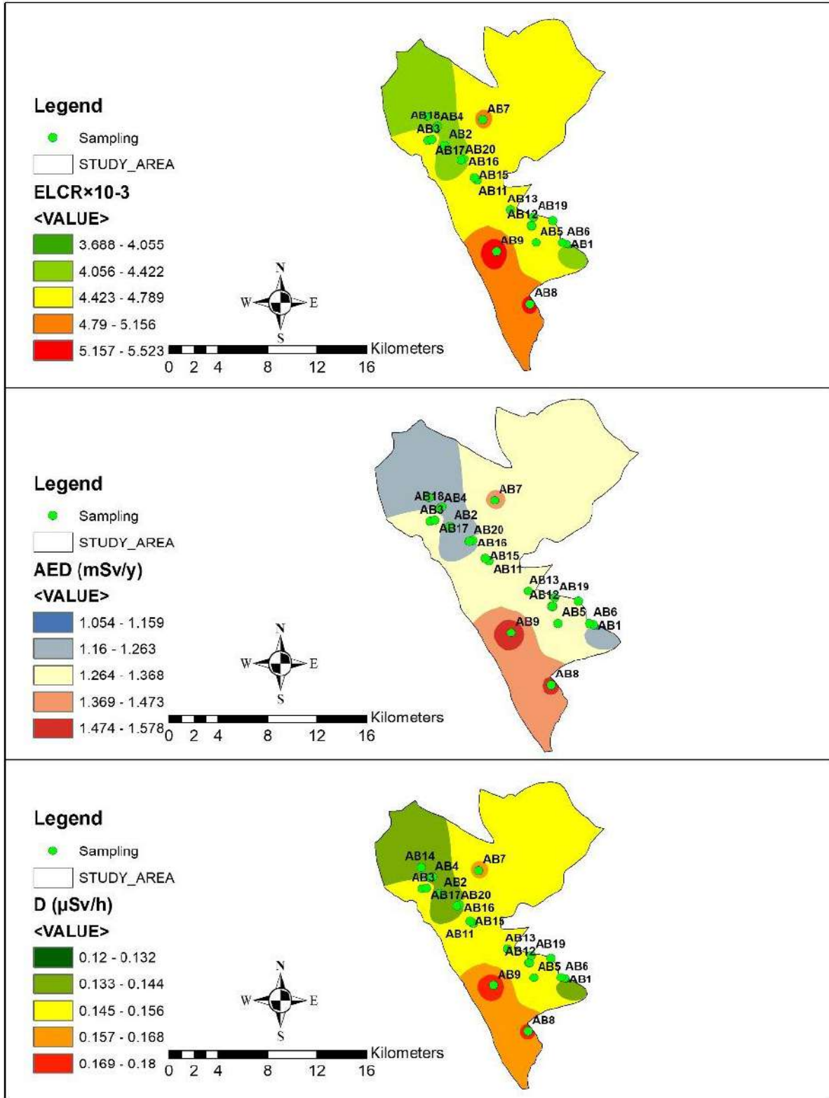
Figure 6. Maps of D, AED, and ELCR in agriculture soil samples present study.
