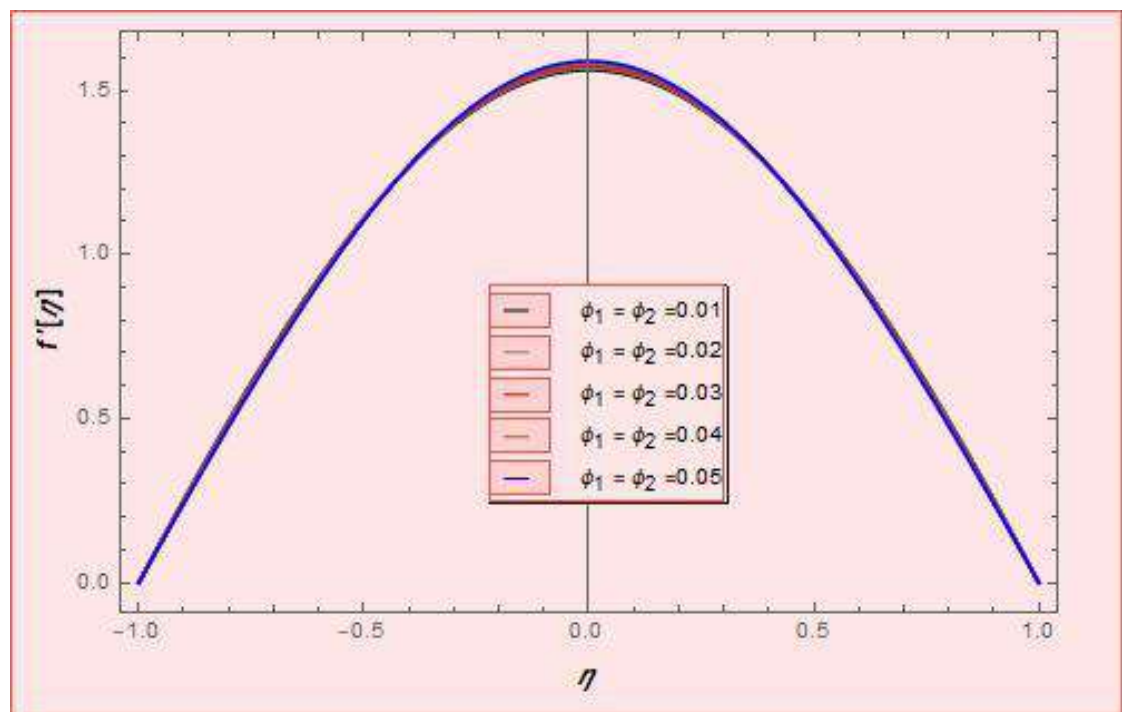
Fig 5; The effect of volume fraction on radial velocity profile.
