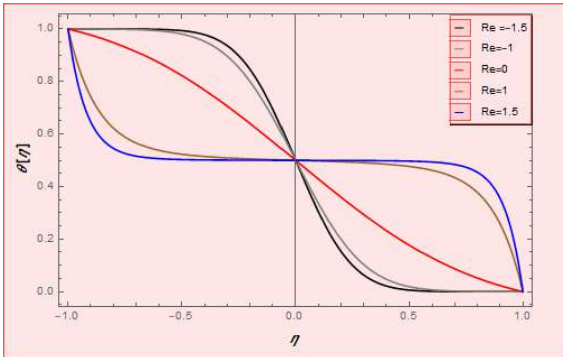
Fig 4; The effect of injection/suction parameter on temperature profile.
