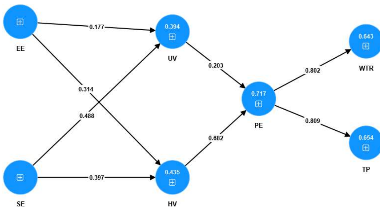
Figure- 2 Path analysis
