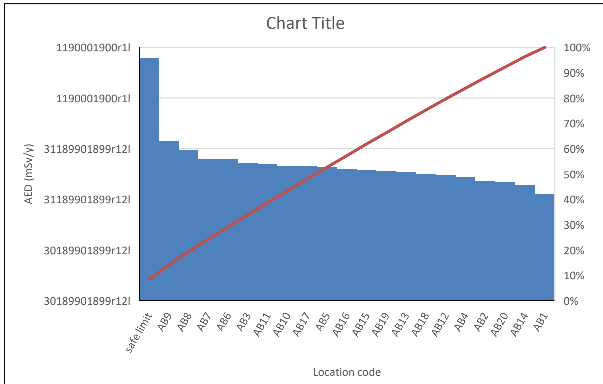
Figure 4. Comparison of the results of AED with safe limit.
